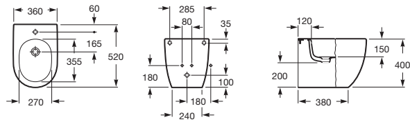
Meridian Wall Faced Bidet
