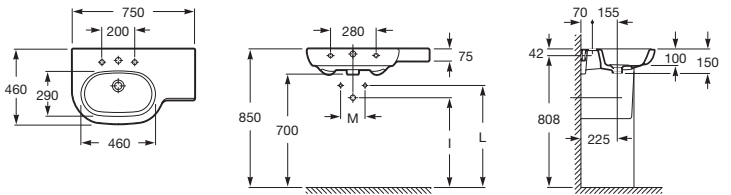
Meridian Wall Basin 750 Left Hand Bowl
