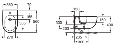
Meridian Wall Hung Bidet
