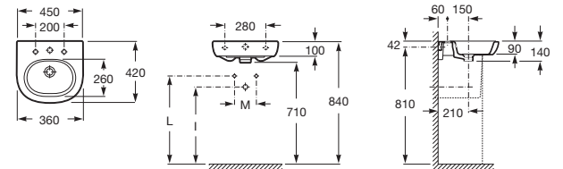
Meridian Wall Basin 750 Left Hand Bowl
