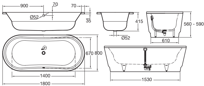
Duo Plus Oval Freestanding
