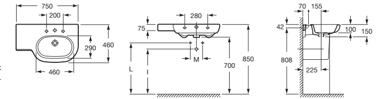
Meridian Wall Basin 750 Right Hand Bowl
