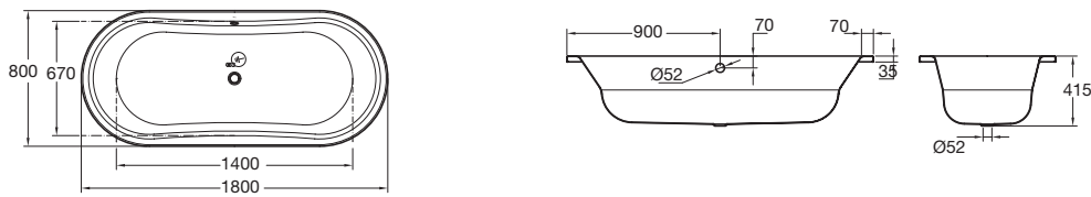
Duo Plus Oval Inset
