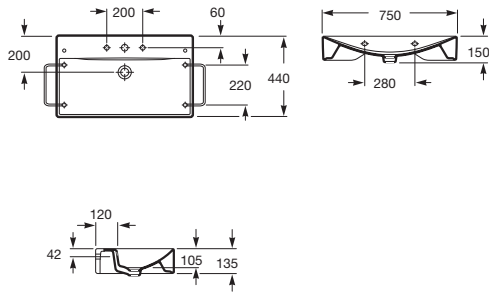
Diverta 750 Wall/Counter Basin
