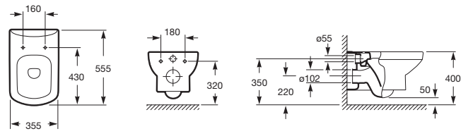
Dama Senso Compact Wall Hung Pan
