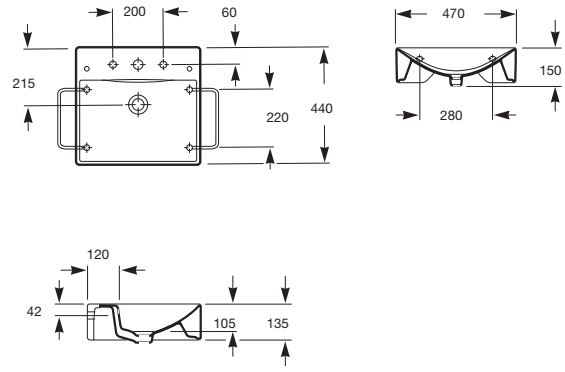
Diverta 470 Wall/Counter Basin
