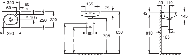
Meridian Wall Basin 350 Cloakroom
