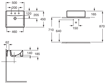
Diverta Semi Recessed Basin
