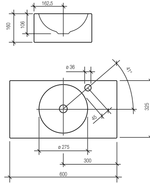
WT7 Wall Basin 6.5 ltr capacity, 1 Taphole 1805908
