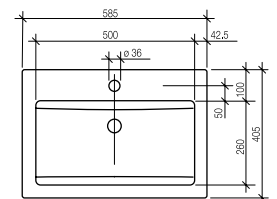
AB 2 585 Semi Inset 5 ltr capacity, 1 Taphole 1805897
