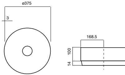
Unisono Counter Basin 375 10 ltr capacity, No taphole 9503960
