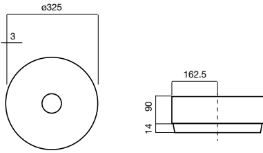
Unisono Counter Basin 325 7 ltr capacity, No taphole 9503961
