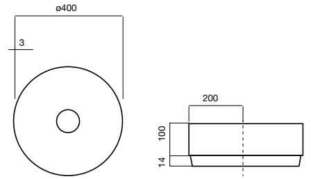
Unisono Counter Basin 400 11.5 ltr capacity, No taphole 9503959
