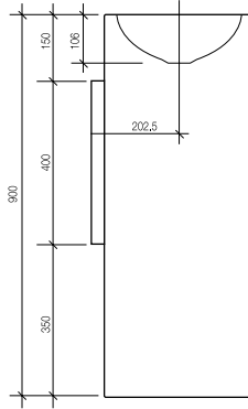
Square Washstand 325 4.5 ltr capacity 1805888
