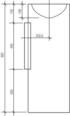
Round Washstand 325 6.5 ltr capacity 1805905
