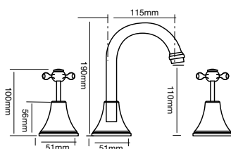
A Basin Set
