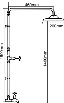
E Exposed Bath/Shower
