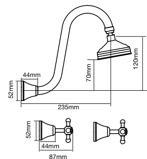
I Deluxe Gooseneck Shower Set
