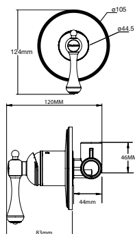
K Bath/Shower Mixer
