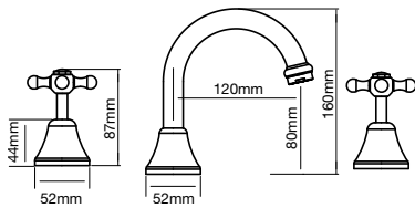
A Basin Set with Fixed Outlet
