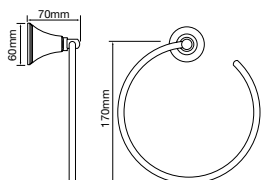
E Towel Ring
