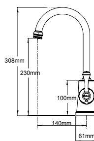
L Sink Mixer Small
