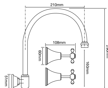
C Wall Sink Set
