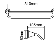
J Double Guest Towel Rail
