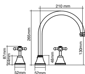
F Hob Sink Set with Swivel Outlet
