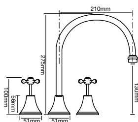
D Hob Spa Set
