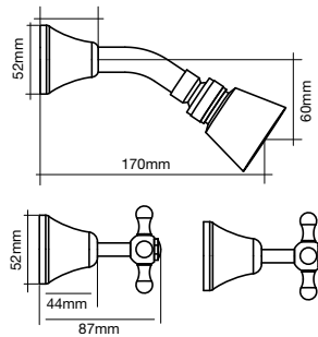
B Shower Set
