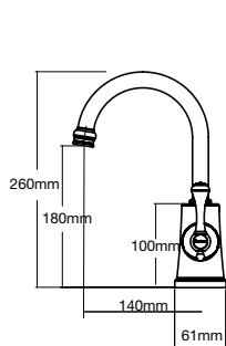
J Basin Mixer
