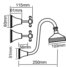
A Fixed Gooseneck Shower Set
