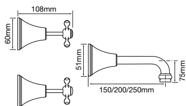
G Bath Set
