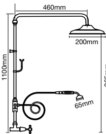
F Exposed Telephone Shower Set
