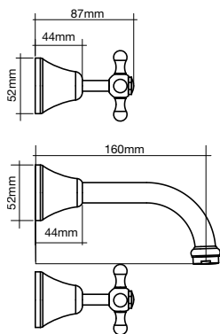
D Bath Set
