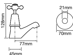
H Pillar Taps
