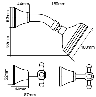
C Deluxe Shower Head on Arm
