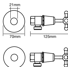
H Washing Machine Stops
