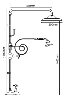
G Exposed Telephone Bath/Shower Set
