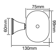
B Soap Dish
