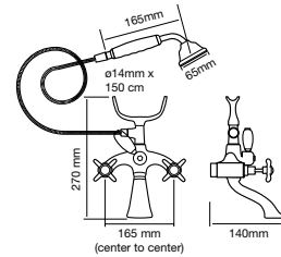
C Telephone style Bath Diverter Hob Mounted
