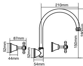
E Wall Sink Set with Swivel Outlet
