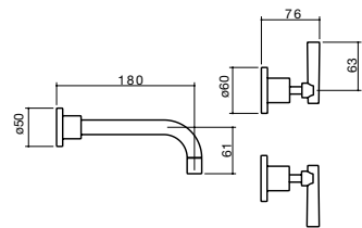
2 Bath Set
