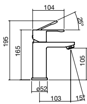
2 Basin Mixer
