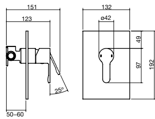
3 Basin/shower Mixer
