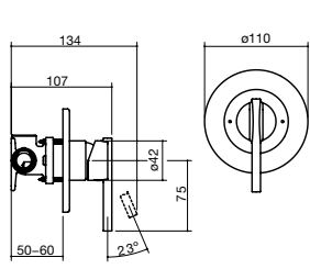
1 Shower/Bath Mixer
