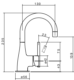
9 Basin Mixer
