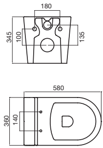
LUX WALL HUNG PAN
