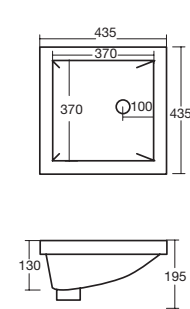
ARC UNDERCOUNTER BASIN 430
