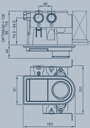
TAHI SINGLE THERMOSTATIC MIXER
