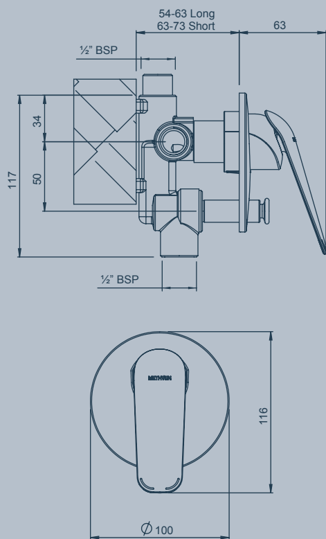
AROHA SHOWER MIXER WITH DIVERTER
